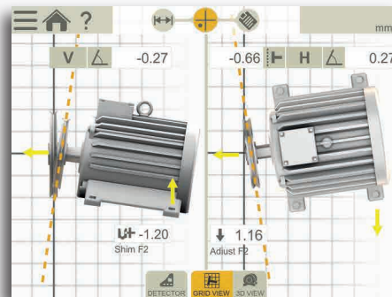
Align machine in live mode, document result with PDF. (XT Alignment app Belt application.)
